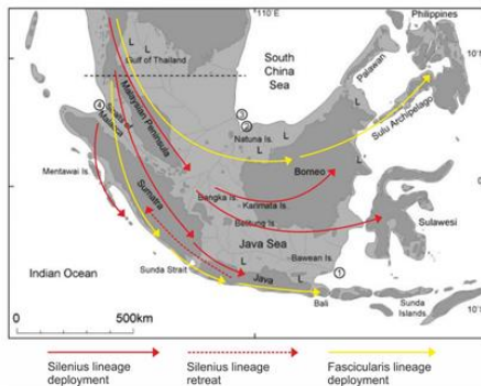
Figure 1. Putative route map of ancient Indonesian NHPs migration 31 Sundaland map is taken from Bird et al. 34
